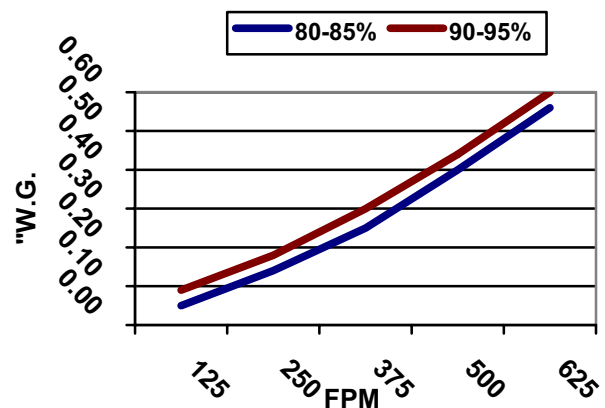
15" Deep Resistance to Airflow
