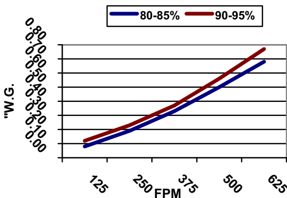
12" Deep Resistance to Airflow
